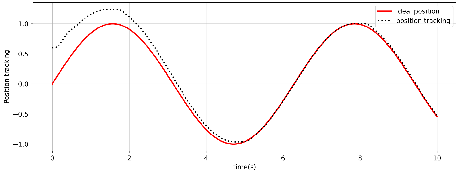
Tracking Performance ( S=3 , S1=1 , m=19 )
